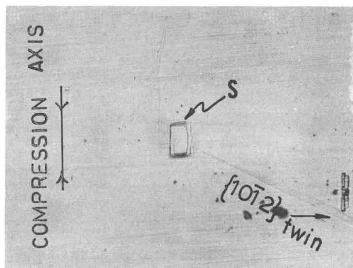
Fig. 4 - Optical Photomicrograph Showing Rectangular Marking at S at the Top of \{10\bar{1}2\} Twin of Crystal ISR-10. Mag. 240X
